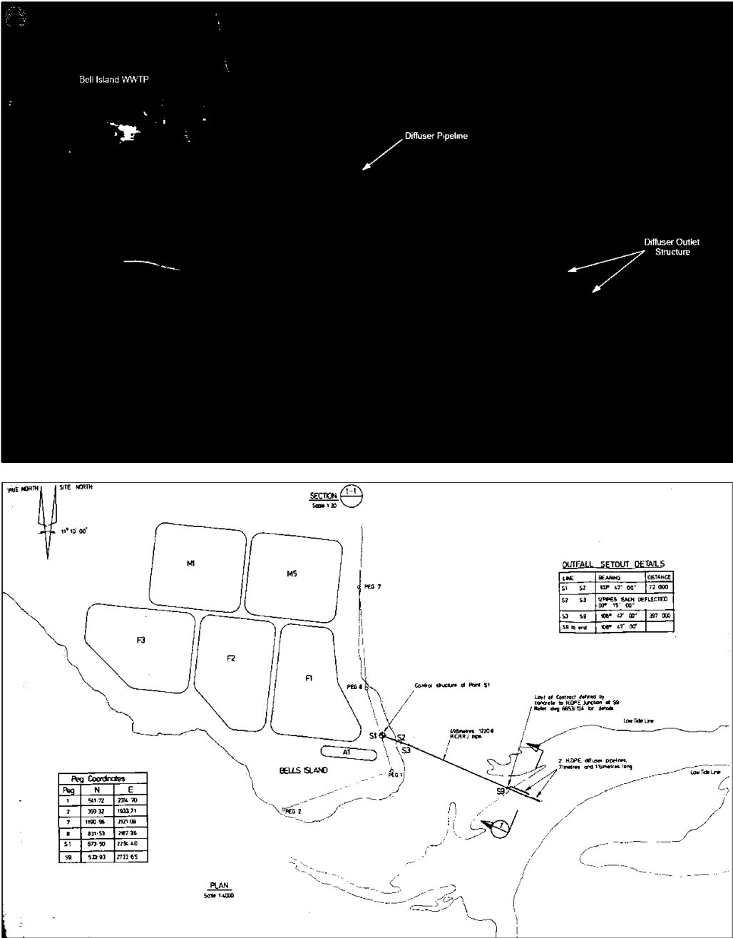
Figure 3. Location of pipe and outlet diffuser structure.
